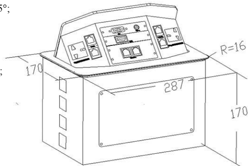
Overall Dimension ( mm )
